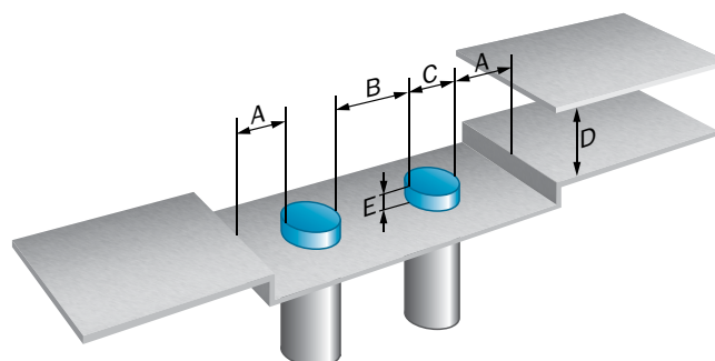
Non-flush installation
