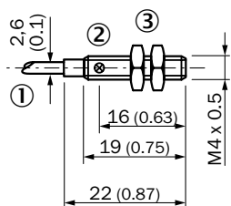
IM04, cable
